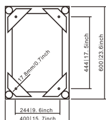
HT6040直架 STRAIGHT SEGMENT
