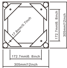
FTB-L 直架 STRAIGHT SEGMENT
