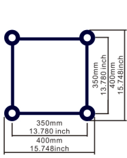
F44直架 BOX STRAIGHT SEGMENT
